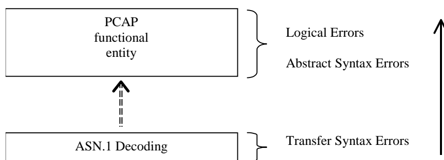
Figure 10: Protocol Errors in PCAP
