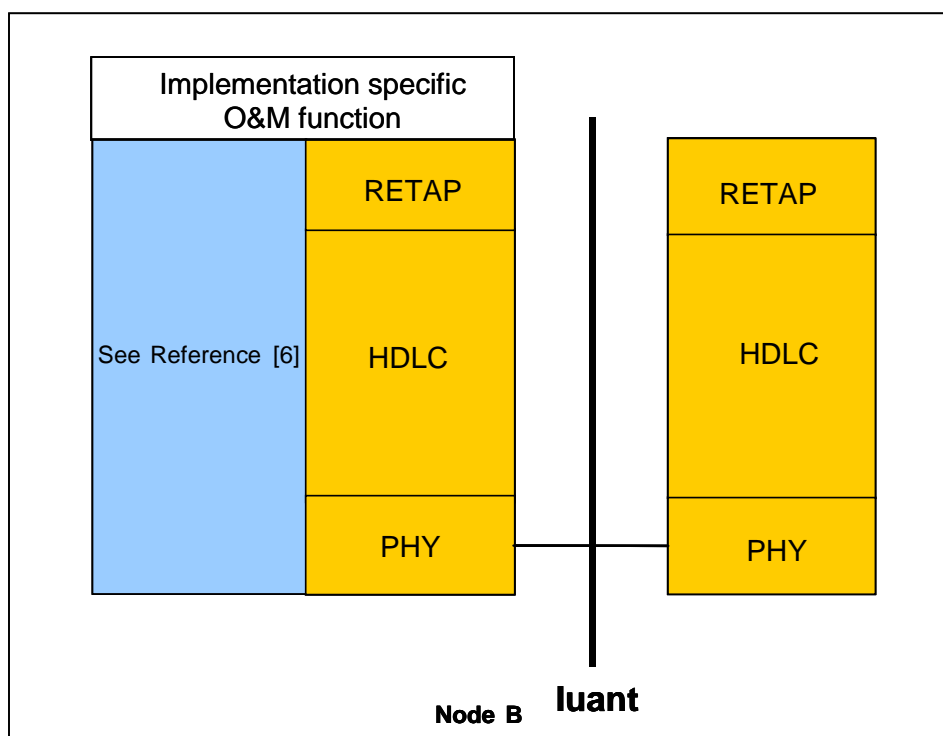
Figure 4.1: Protocol Structure for Iuant interface
