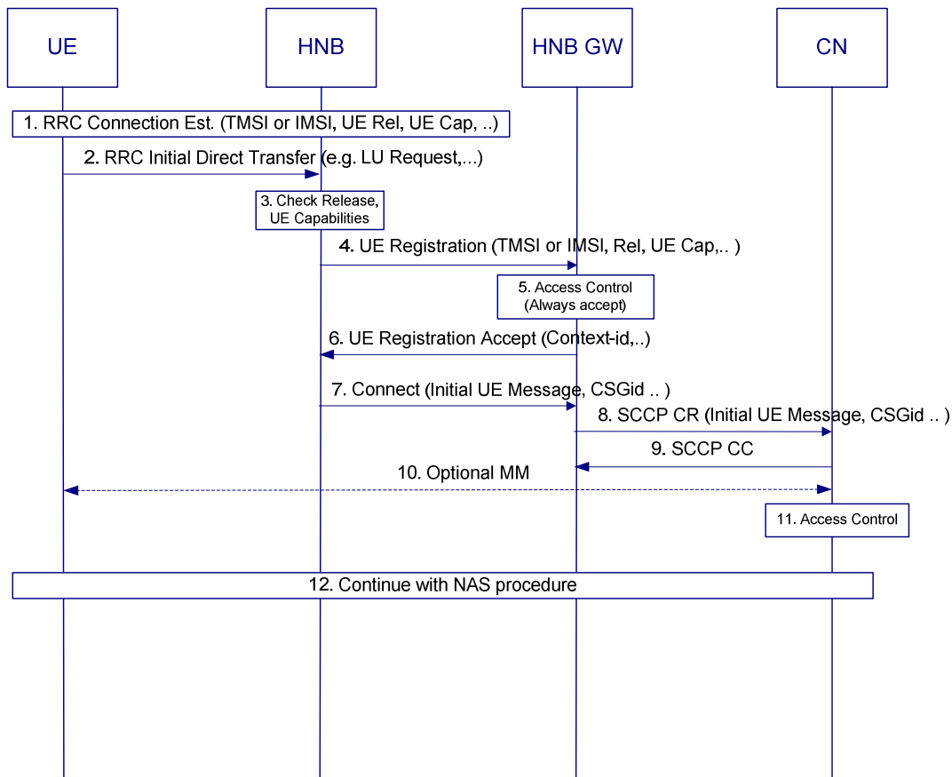
Figure 5.1.3-1. UE Registration for Rel-8 UEs.
