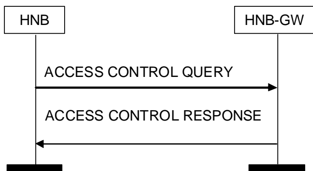
Figure 12: Access Control Query Procedure: Successful Operation
