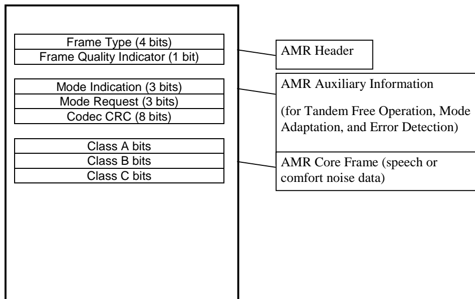
Figure 1. Generic AMR frame structure
