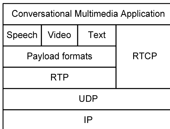
Figure 4.3: User plane protocol stack for a basic MTSI client
