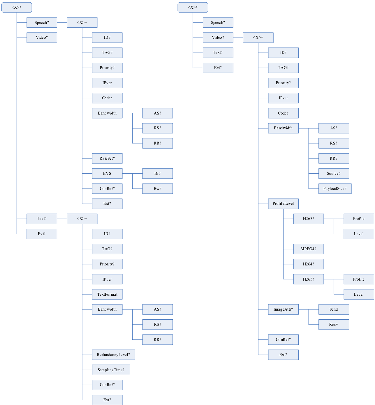
Figure 15.1: MTSI network preference management object tree
