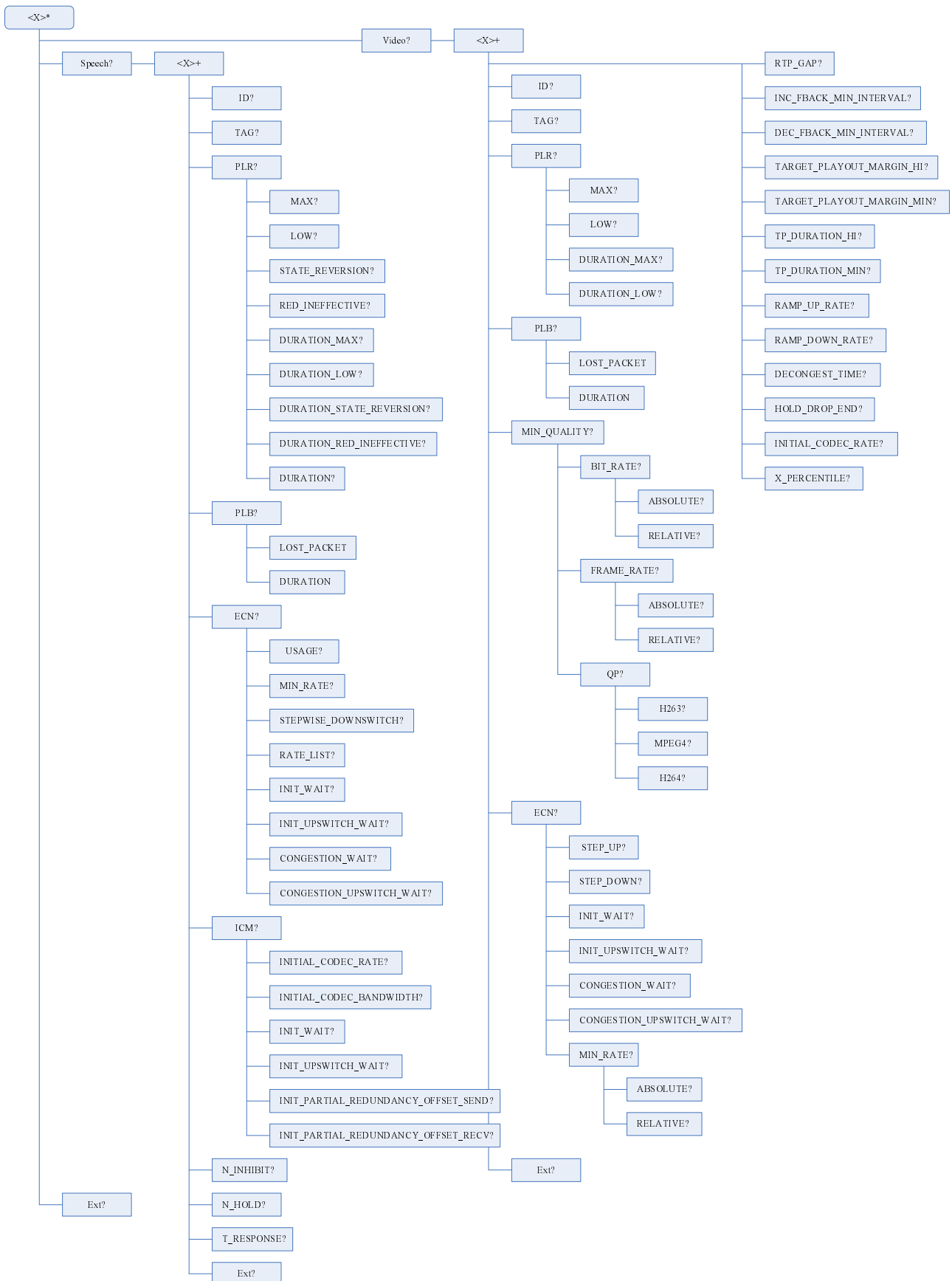
Figure 17.1: MTSI media adaptation management object tree
