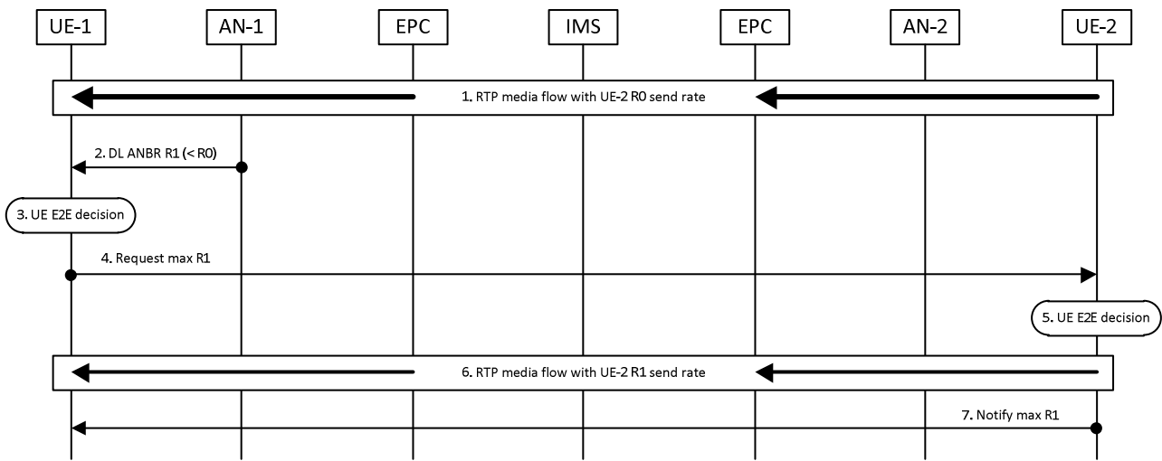
Figure 10.7-3 Downlink bitrate decrease based on ANBR through application signaling
