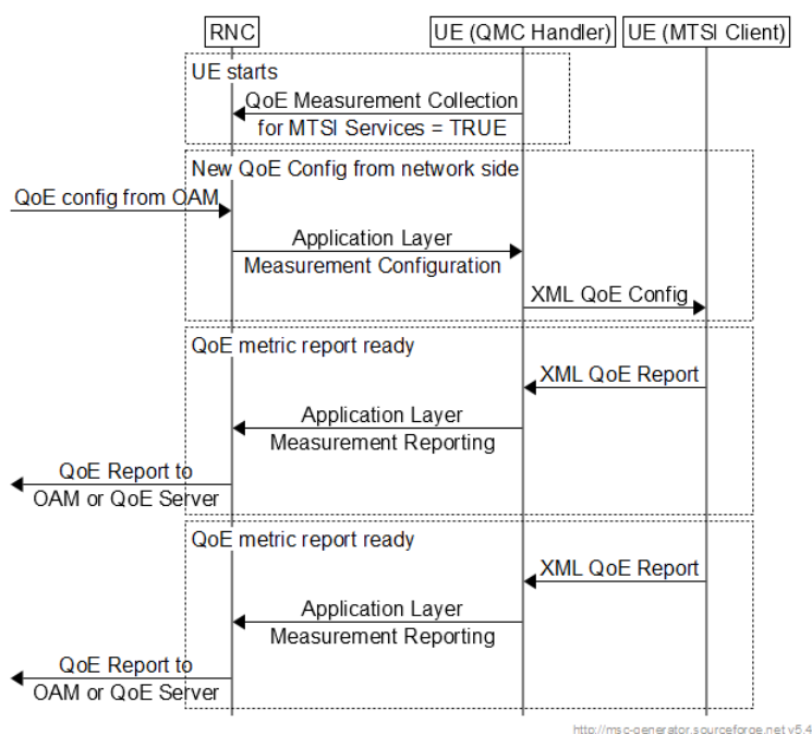
Figure L-1: Example signalling diagram for UMTS
