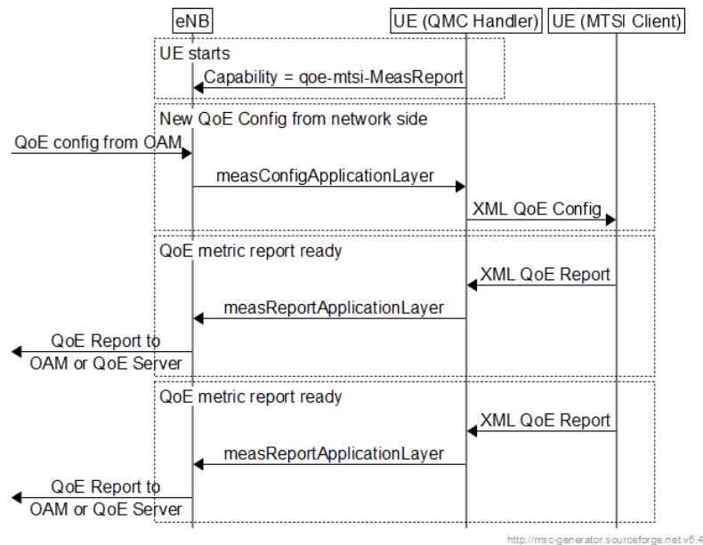
Figure L-2: Example signalling diagram for LTE
