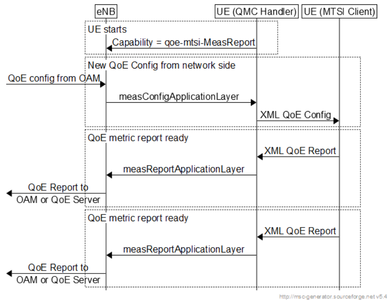
Figure 16.5.1-2: Example signalling diagram for LTE
