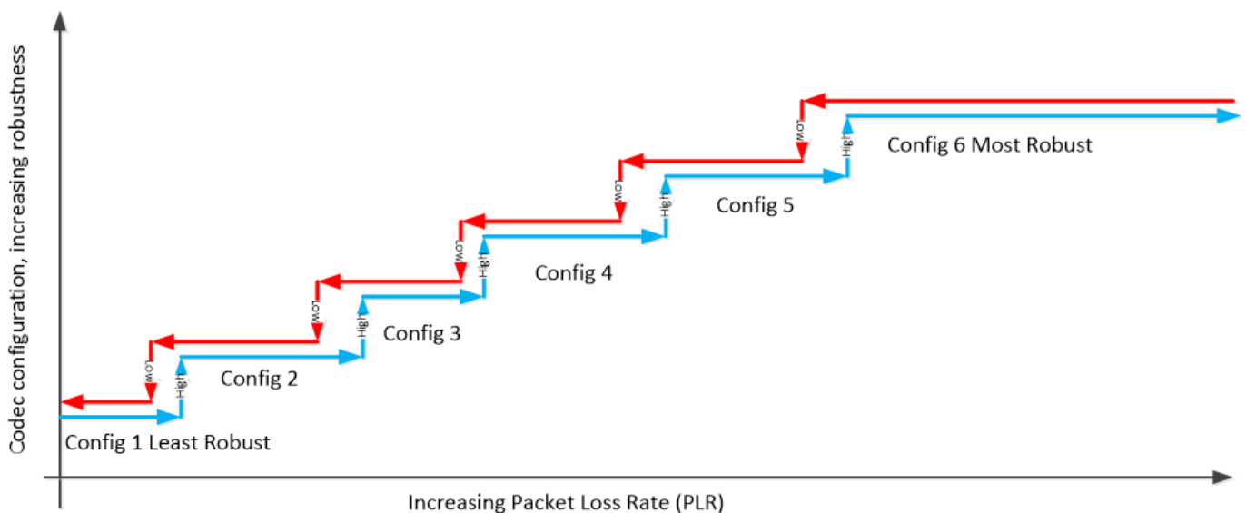
Figure 17.2: High and Low PLR thresholds for media robustness adaptation
