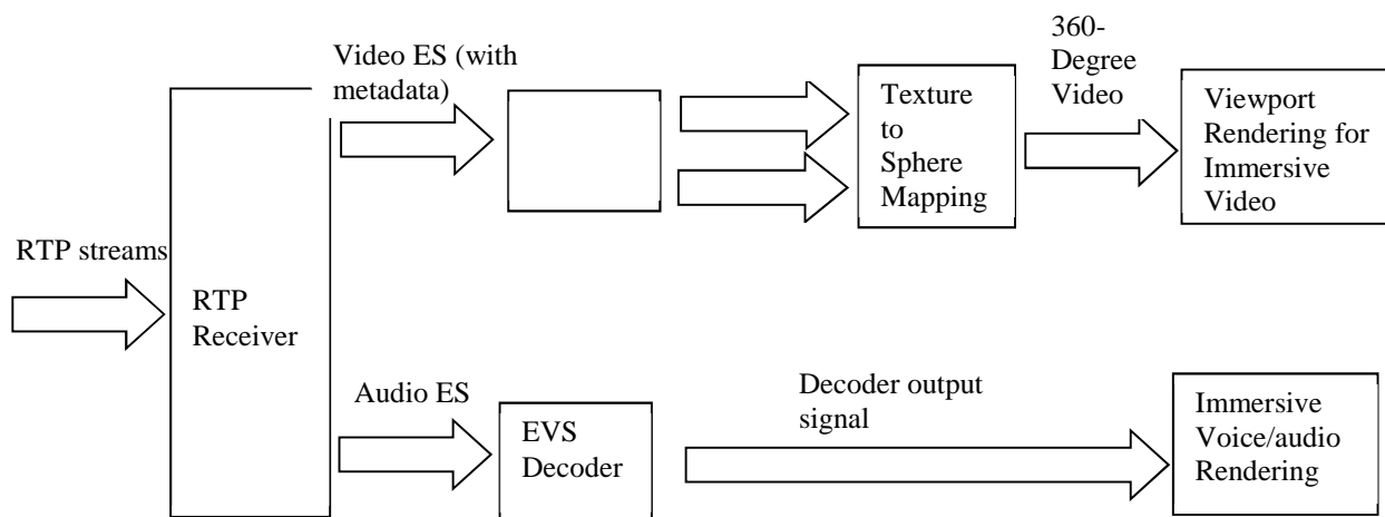
Figure Y.2: Reference receiver architecture for ITT4RT-client in terminal. The output signal, i.e., the decoded picture or "texture", is then rendered using the Decoder Metadata information in relevant SEI messages contained in the video elementary streams as well as the relevant information signalled at the RTP/RTCP level (in the viewport-dependent case). The Decoder Metadata is used when performing rendering operations such as region-wise unpacking, projection de-mapping and rotation for 360-degree projected video, or fisheye video information for 360-degree fisheye video) toward creating spherical content for each eye. Details of such sample location remapping process operations are described in clause D.3.41.7 of ISO/IEC 23008-2 [119].
