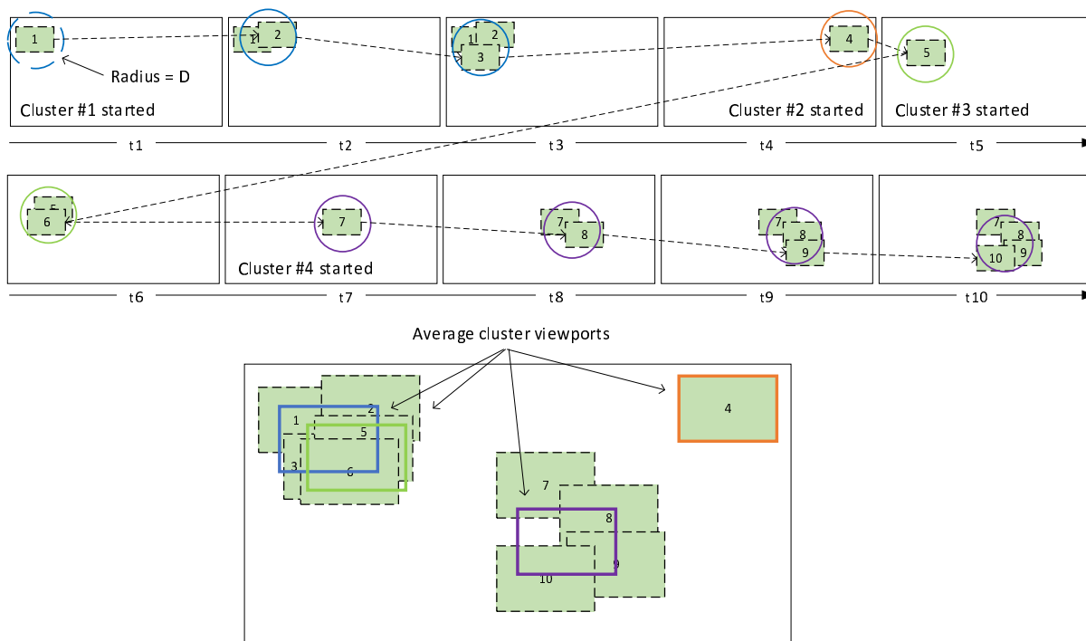
Figure D.2-2 Duration filtering example
