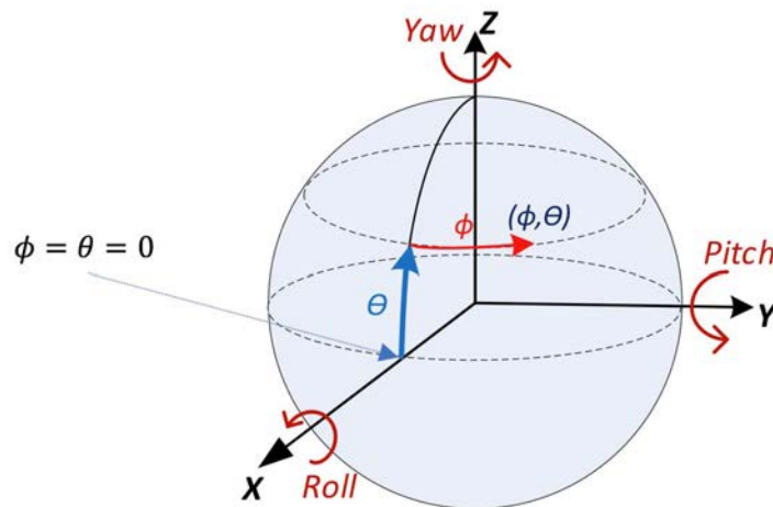
Figure A.1: 3D XYZ coordinate definition
