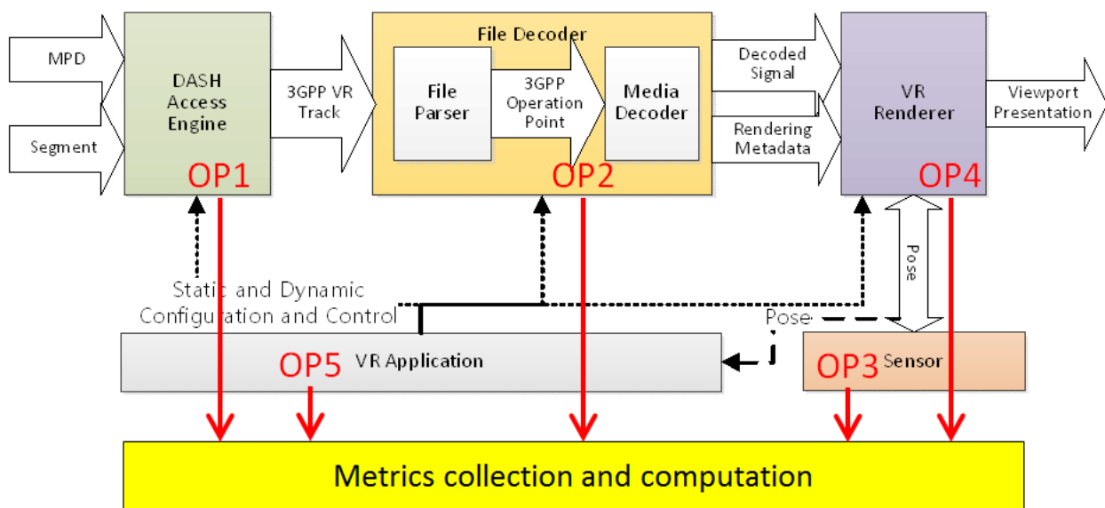
Figure 9.2.1-1: Client reference architecture for VR metrics
