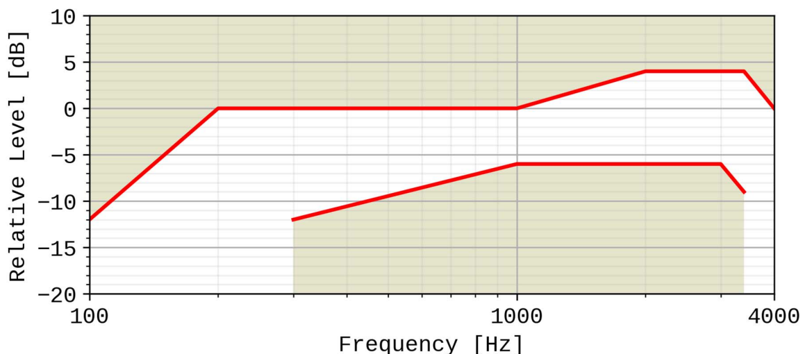
Figure 1: Handset and headset sending sensitivity/frequency mask
