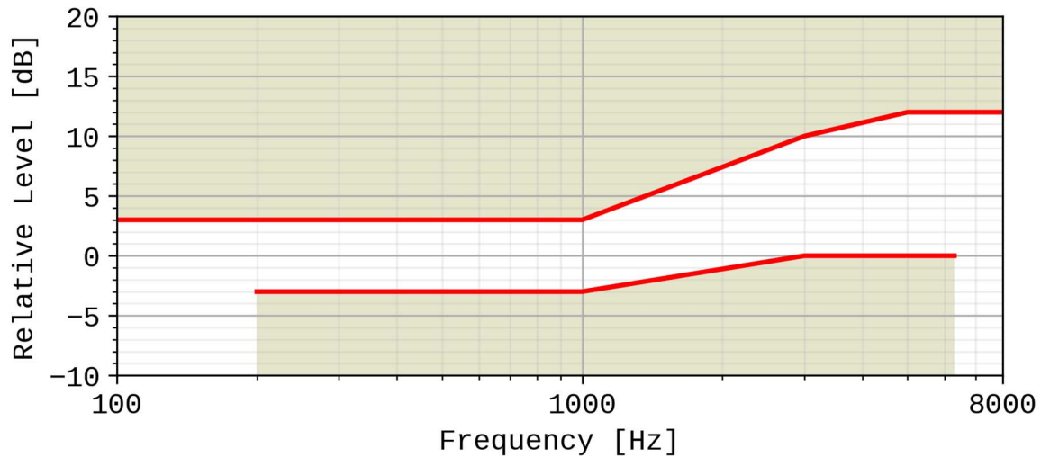
Figure 14a1: Electrical interface sending sensitivity/frequency mask
