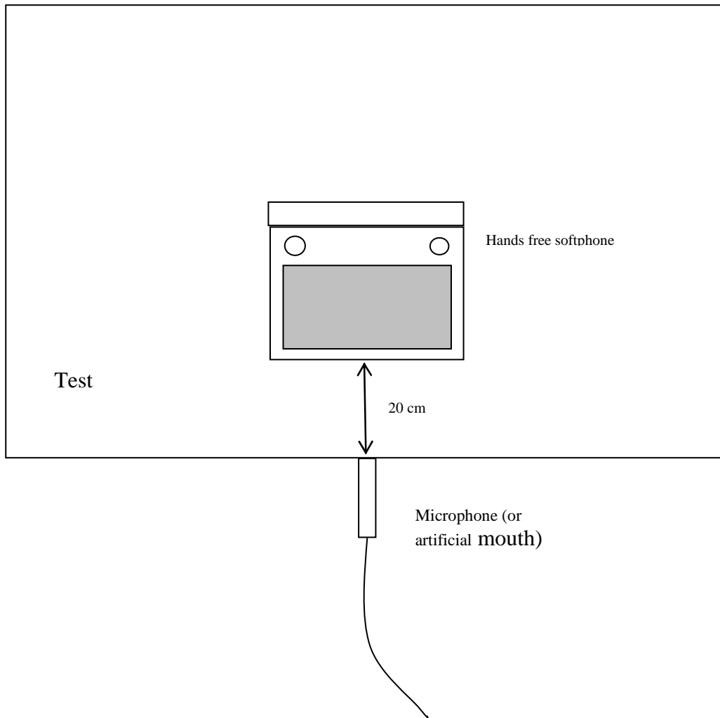
Figure 9: Configuration of softphone relative to the free field microphone or artificial mouth top view
