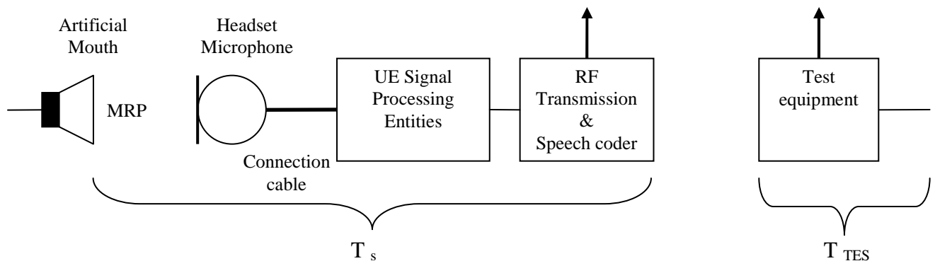
Figure 19b2: Different entities when measuring the delay in sending direction with a headset connected via cable
