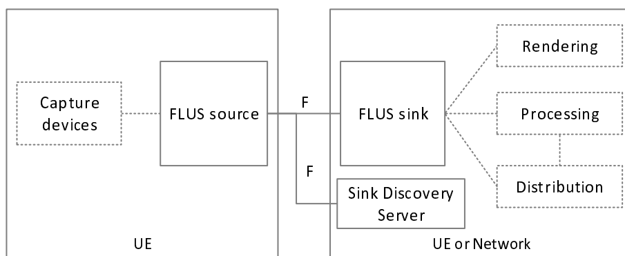
Figure 4.2-1: FLUS architecture
