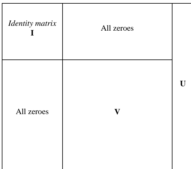
Figure E.2.2-1 – Submatrices of \mathbf{A} in the first phase
