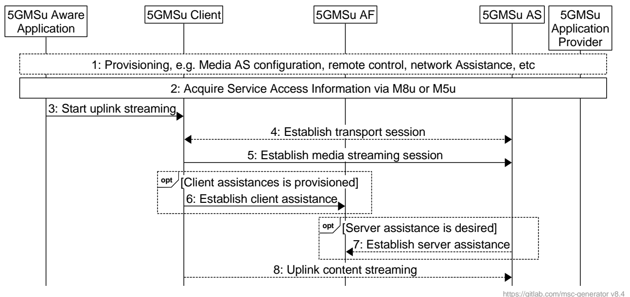
Figure 6.3-1: Uplink Streaming Session Establishment
