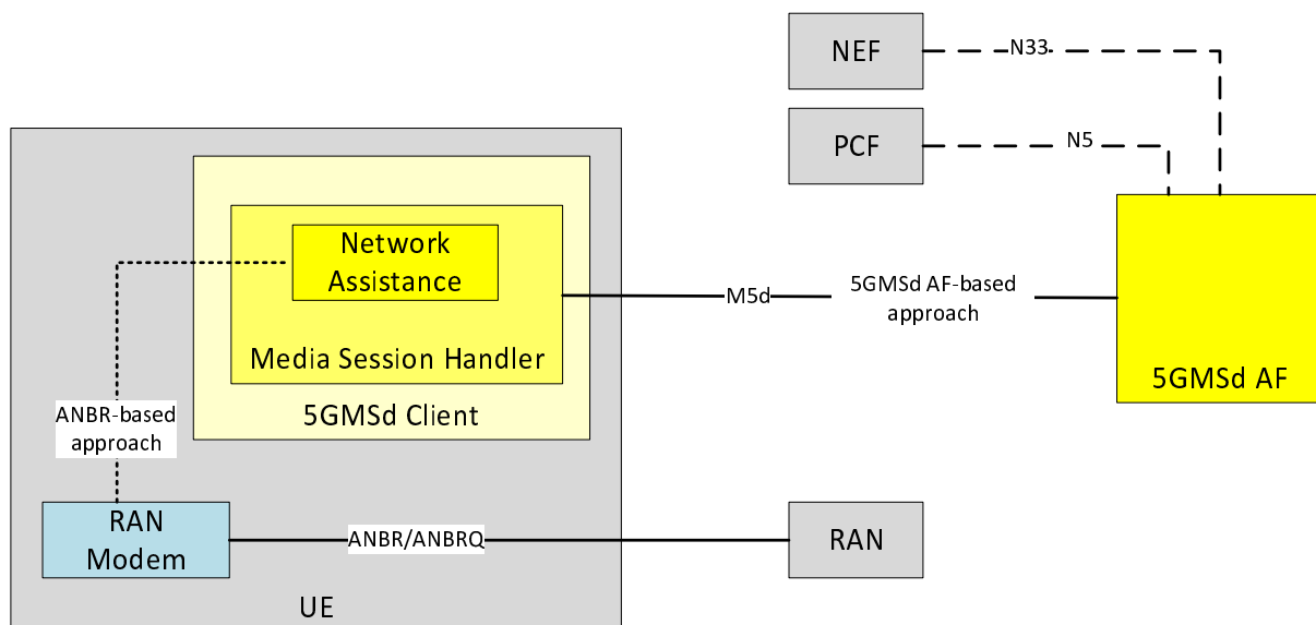
Figure 5.9.1-1: Downlink Network Assistance alternative approaches
