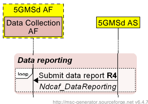
Figure 5.10.2-1: Downlink media streaming access reporting
