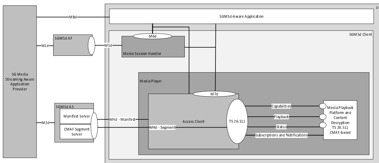
Figure 4.1-1 5G Media Downlink Streaming Architecture
