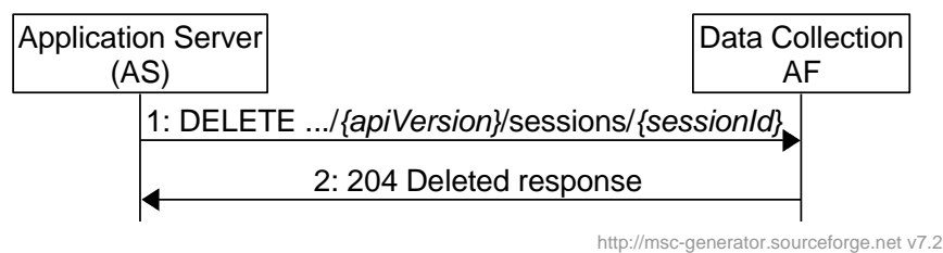
Figure 4.2.5.4-1: Application Server destroys DataReportingSession
