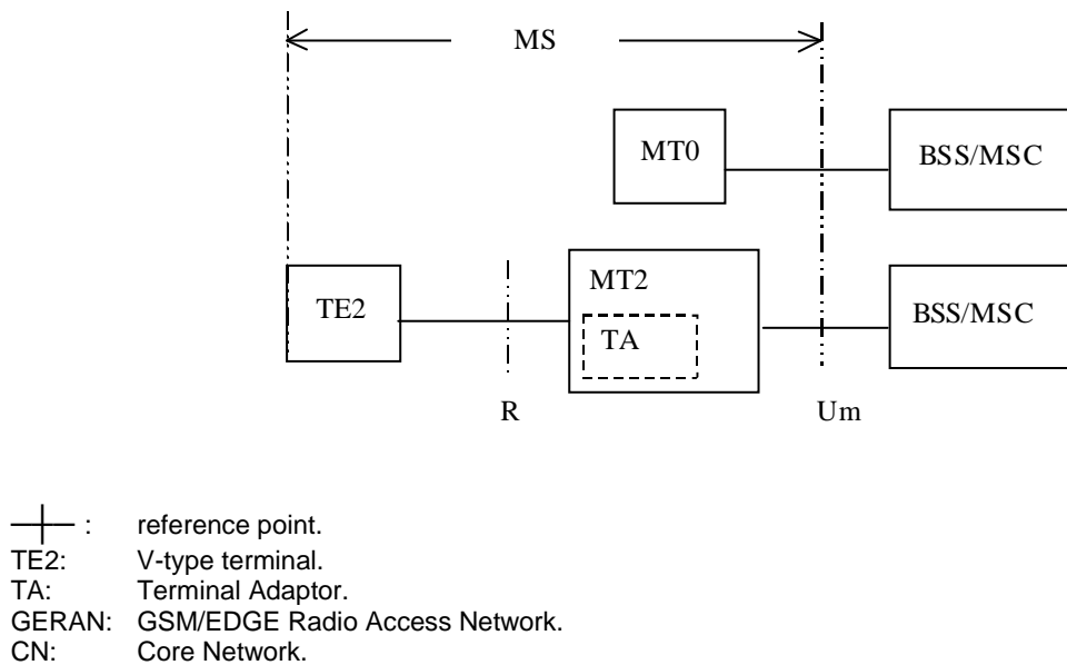
Figure 1: PLMN Access Reference Configuration (in A/Gb mode and GERAN Iu mode)
