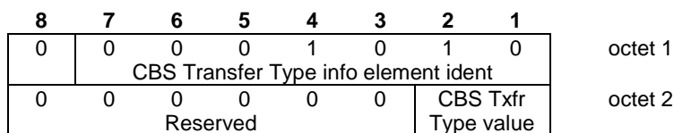
Figure 2.5.12: CBS Transfer Type information element
