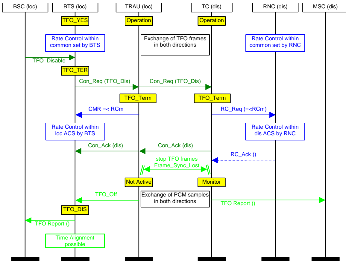
G.3.1-1: TFO_Disable during operation – passive partner: UMTS
