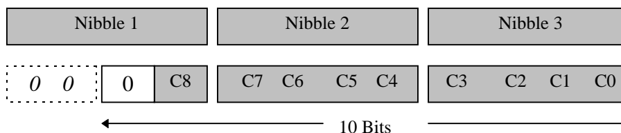
Figure A.1.3-1: General Construction of an IS_Command_Block
