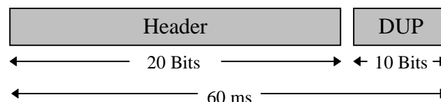
Figure A.2.5-1: Construction of the IS_DUP Message
