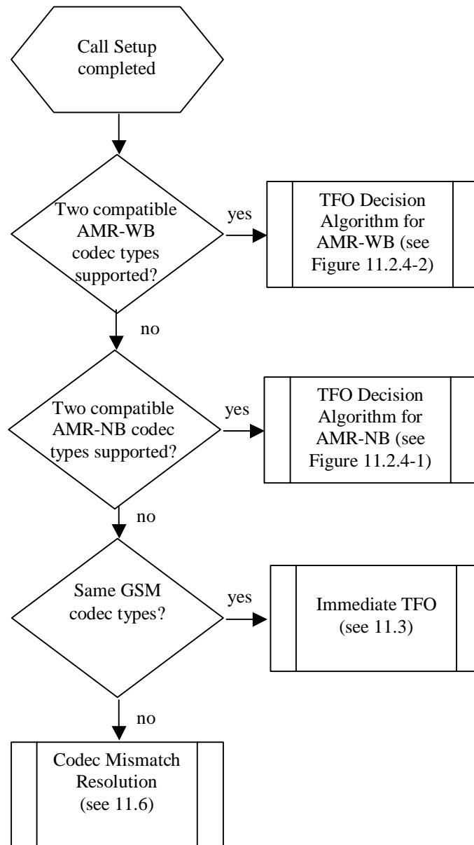
Figure 11.1-1: Main TFO Decision Algorithm
