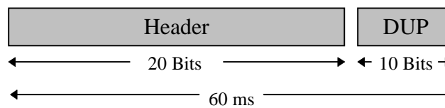
Figure A.2.5-1: Construction of the IS_DUP Message
