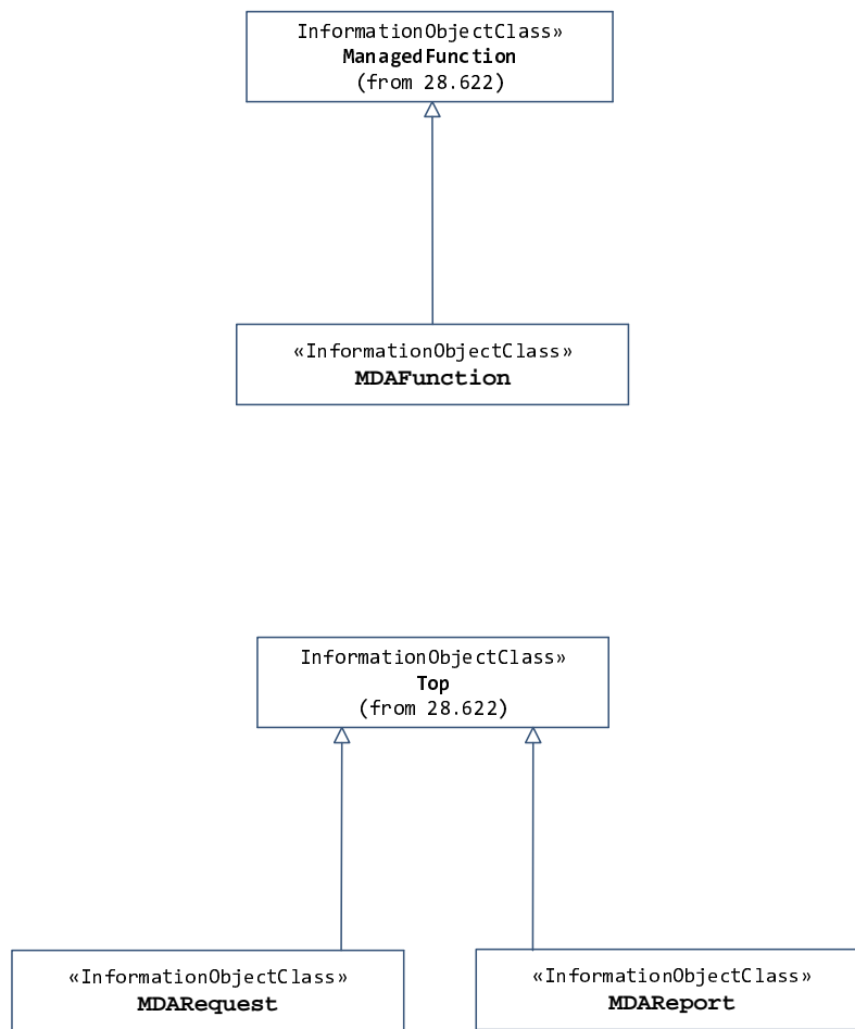
Figure 9.2.2-1: Inheritance Hierarchy
