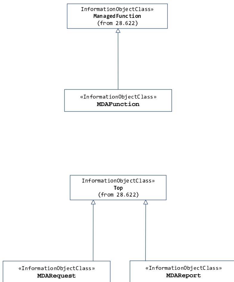
Figure 9.2.2-1: Inheritance Hierarchy
