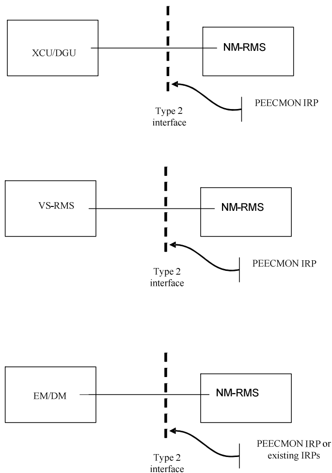
Figure 4.1.1: System Context
