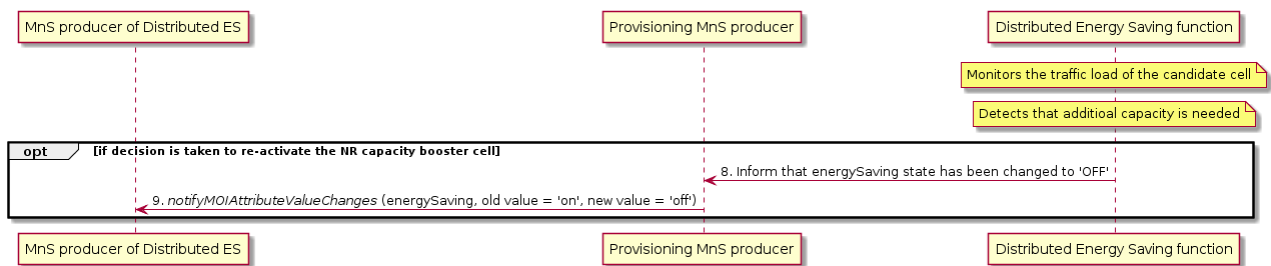
Figure 6.2.3.2-1: Distributed energy saving deactivation
