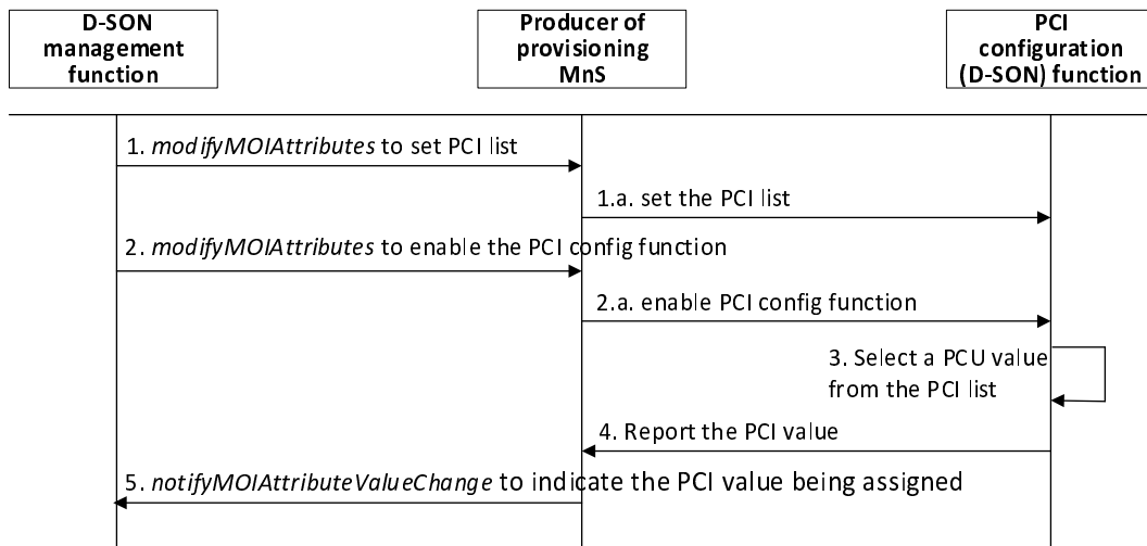
Figure 8.2.3.1-1: Initial PCI configuration procedure
