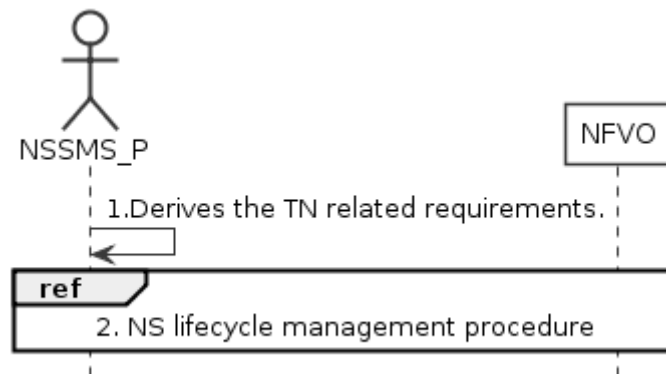
Figure 7.9.2-1: Interaction with NFVO as TN manager to support network slicing
