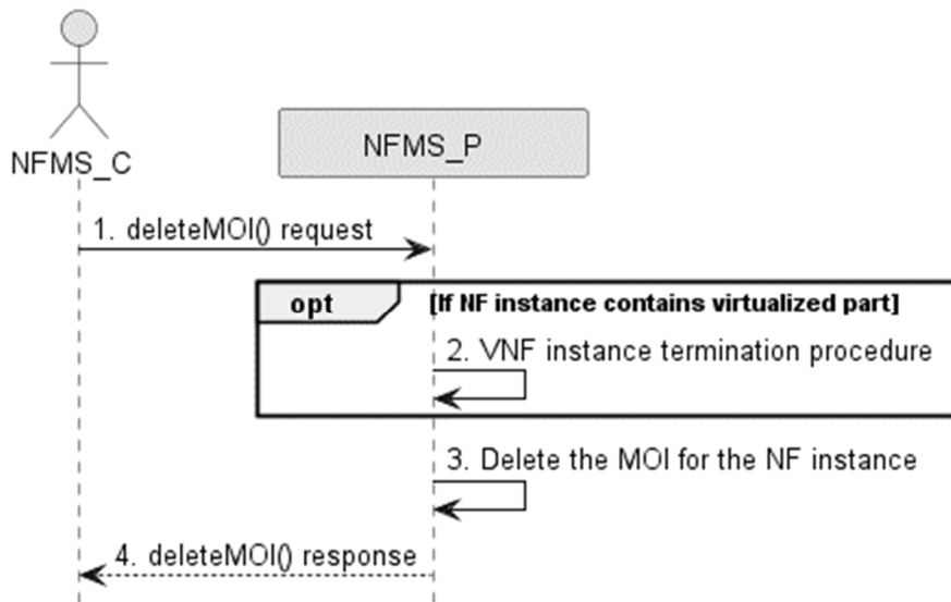
Figure 7.12-1: Network Function Instance Deletion procedure
