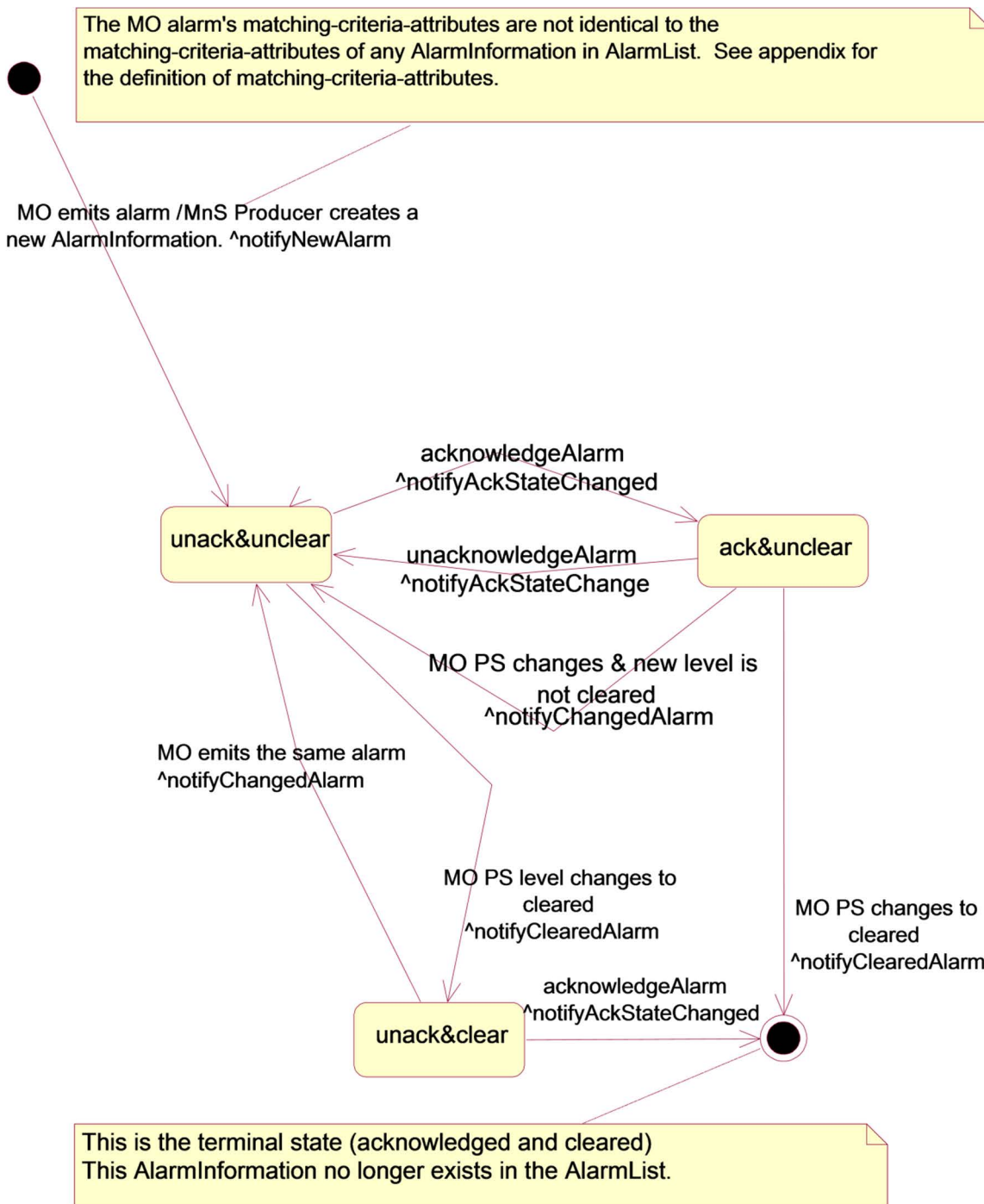
Figure 10.2.2.1.3.1.3-1 notifyChangedAlarm supported
