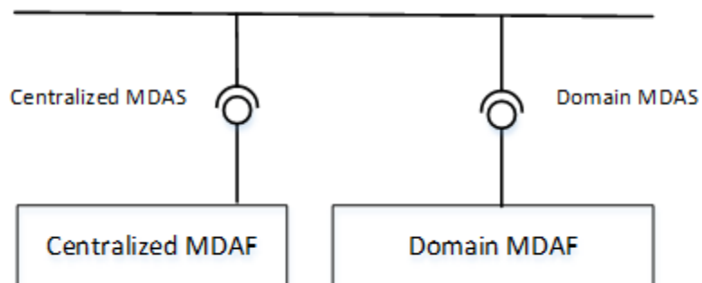
Figure 4.6.1: Service based architecture for management data analytics
