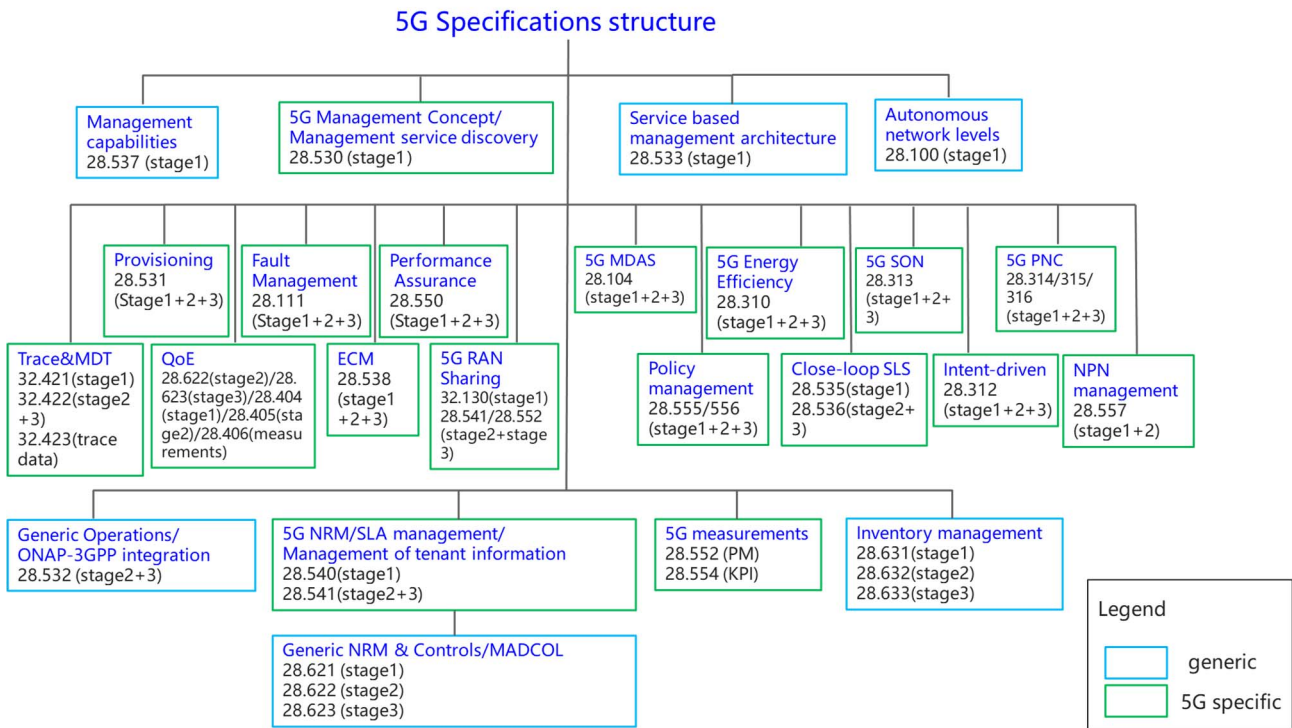
Figure E-1: Overview of 5G management specifications
