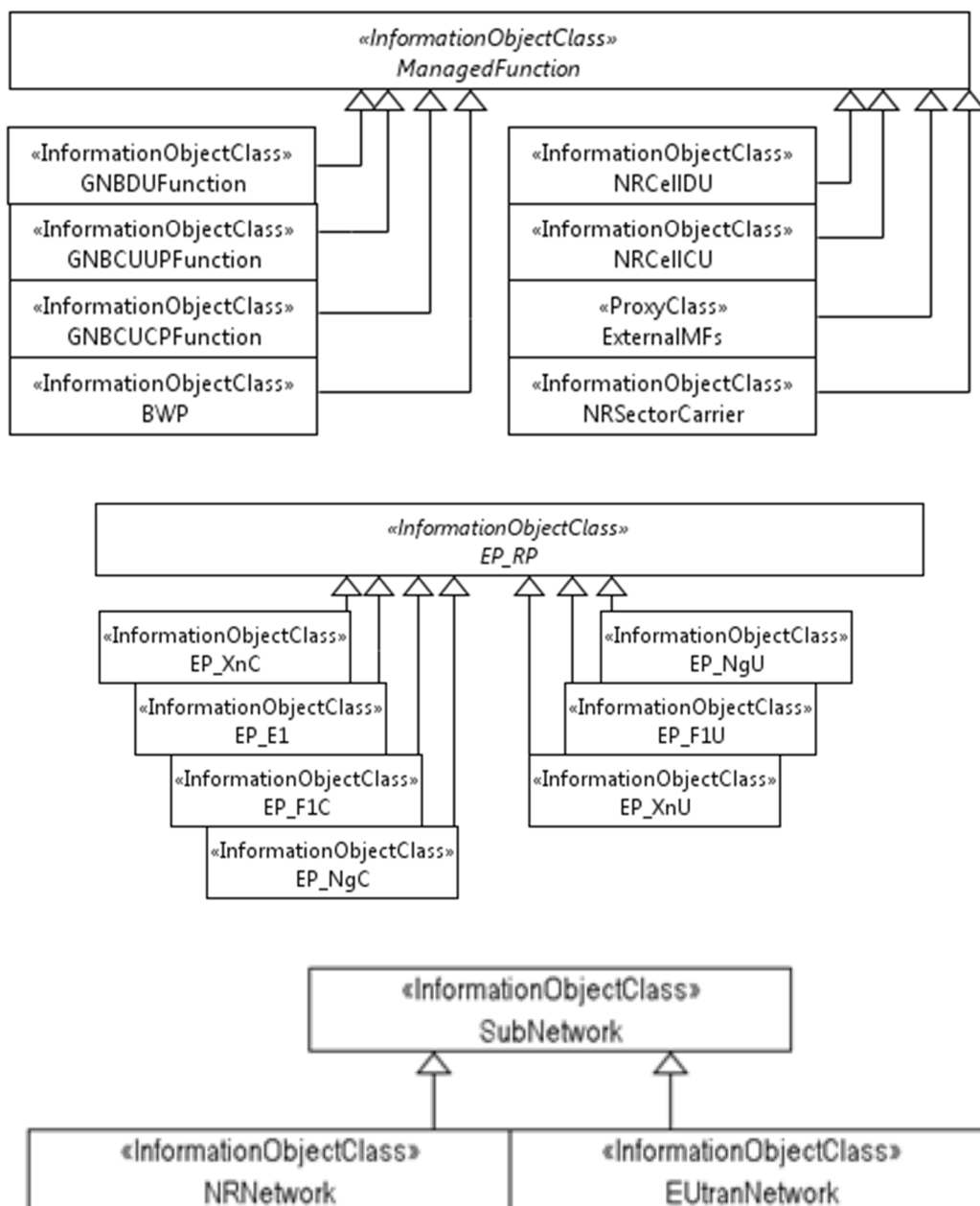
Figure 4.2.1.2-1: Inheritance Hierarchy
