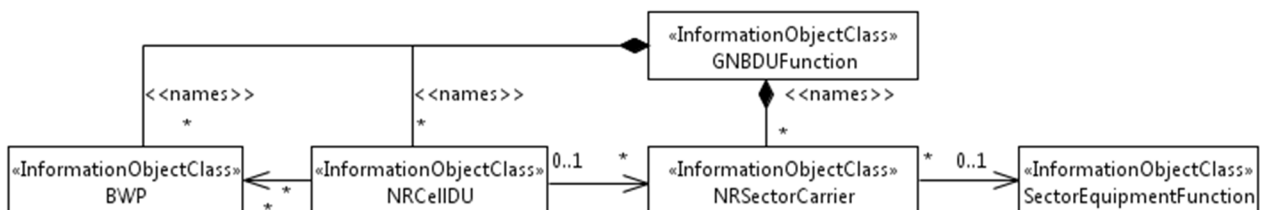
Figure 4.2.1.1-3: NRM for «IOClass»NRSectorCarrier and «IOClass»BWP for all deployment scenarios
