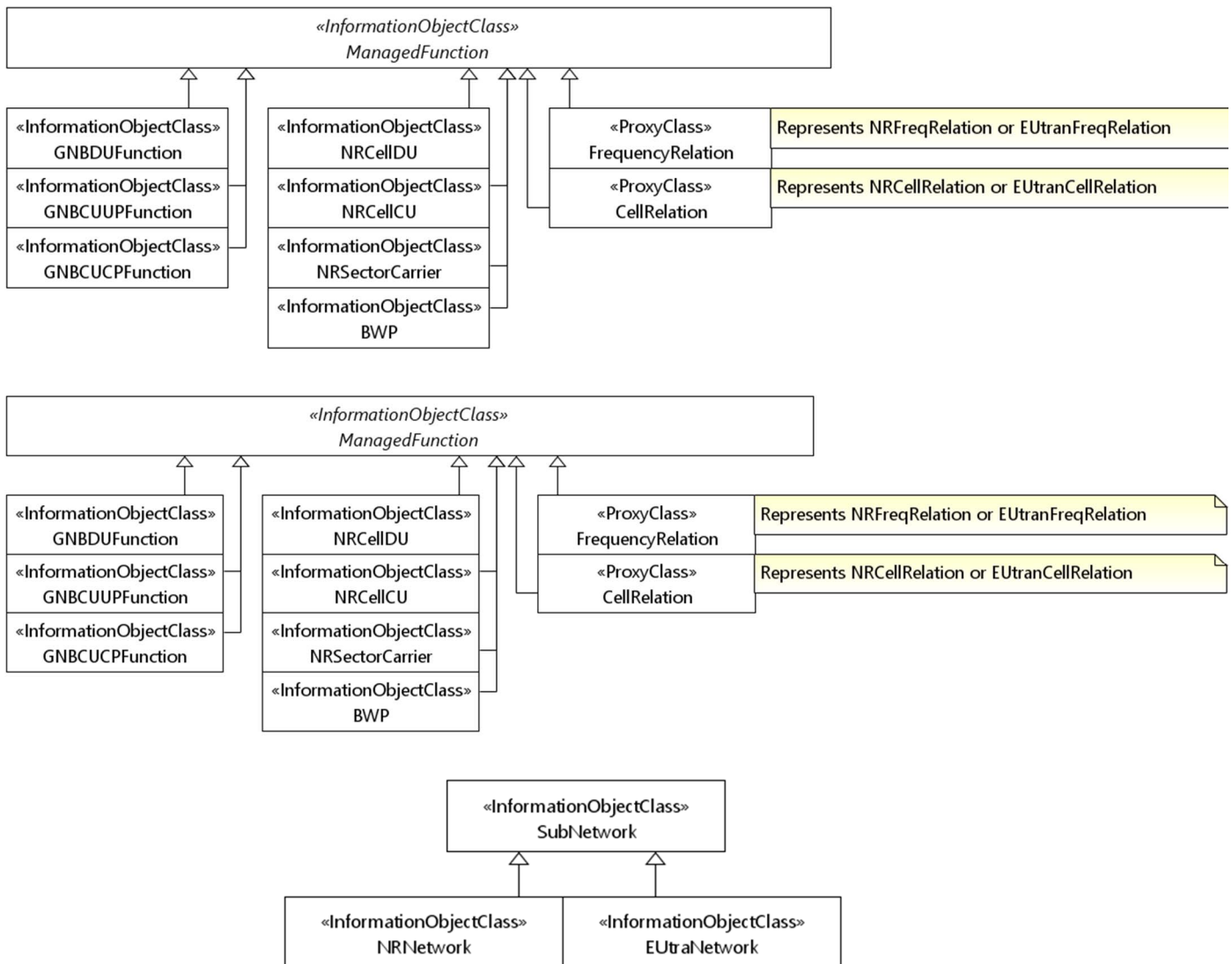
Figure 4.2.1.2-1: Inheritance Hierarchy
