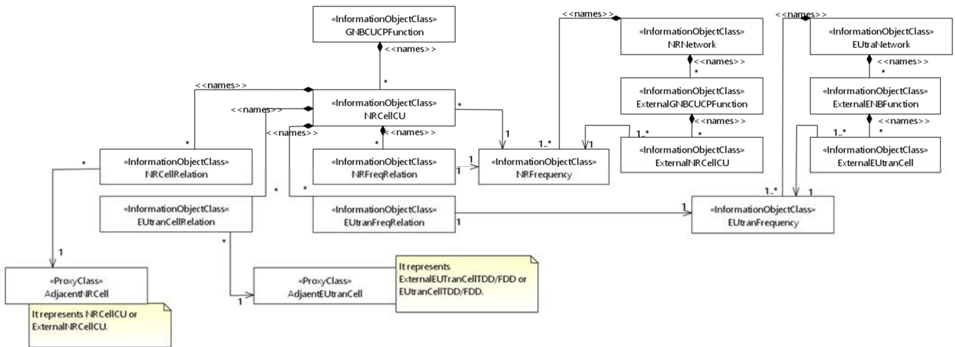
Figure 4.2.1.1-5: Cell Relation view for all deployment scenarios
