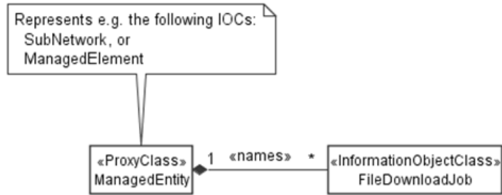
Figure 4.2.1-10: File download NRM fragment
