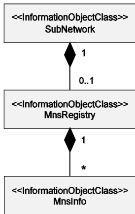
Figure 4.2.1-8: MnS Registry NRM fragment
