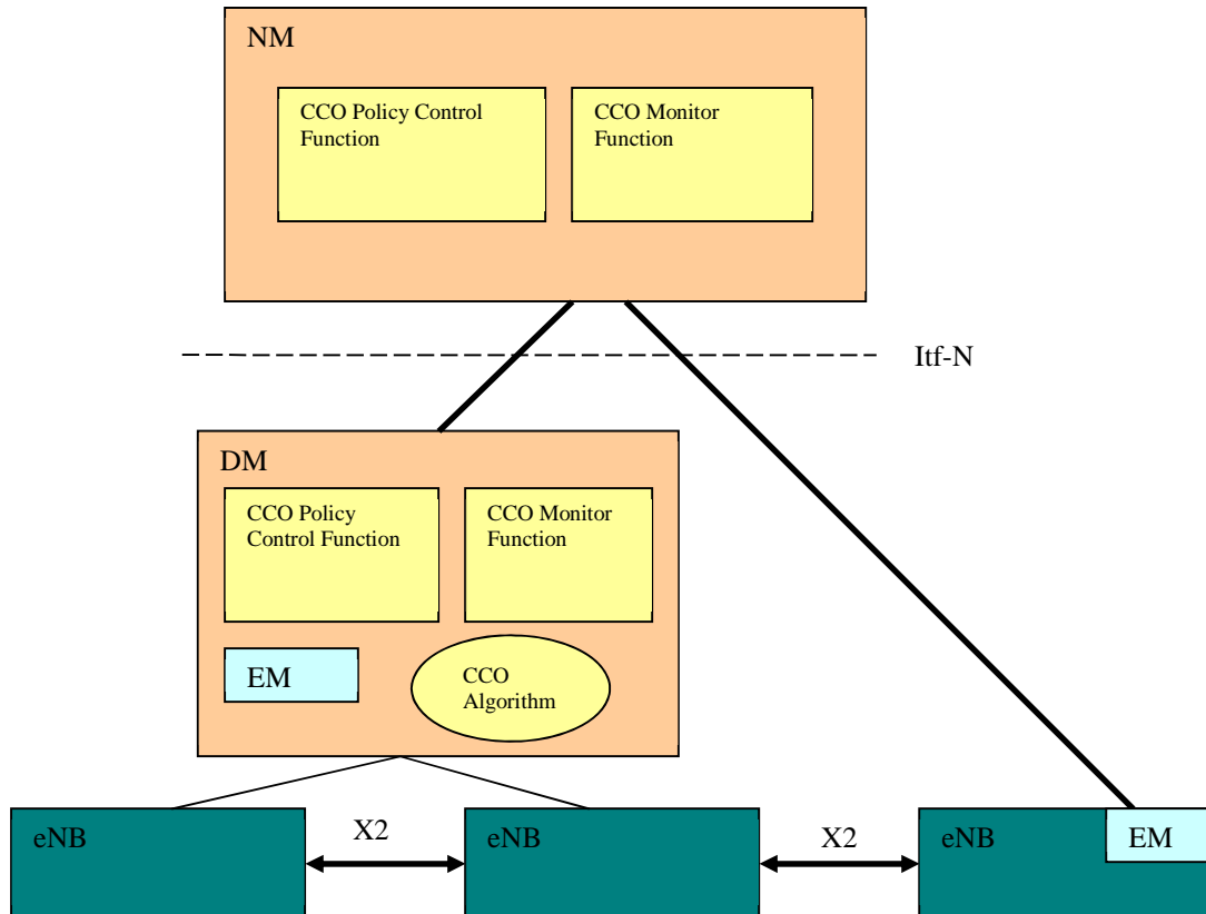
Figure 4.5.4.2-1: Example when the CCO SON algorithm is located in DM
