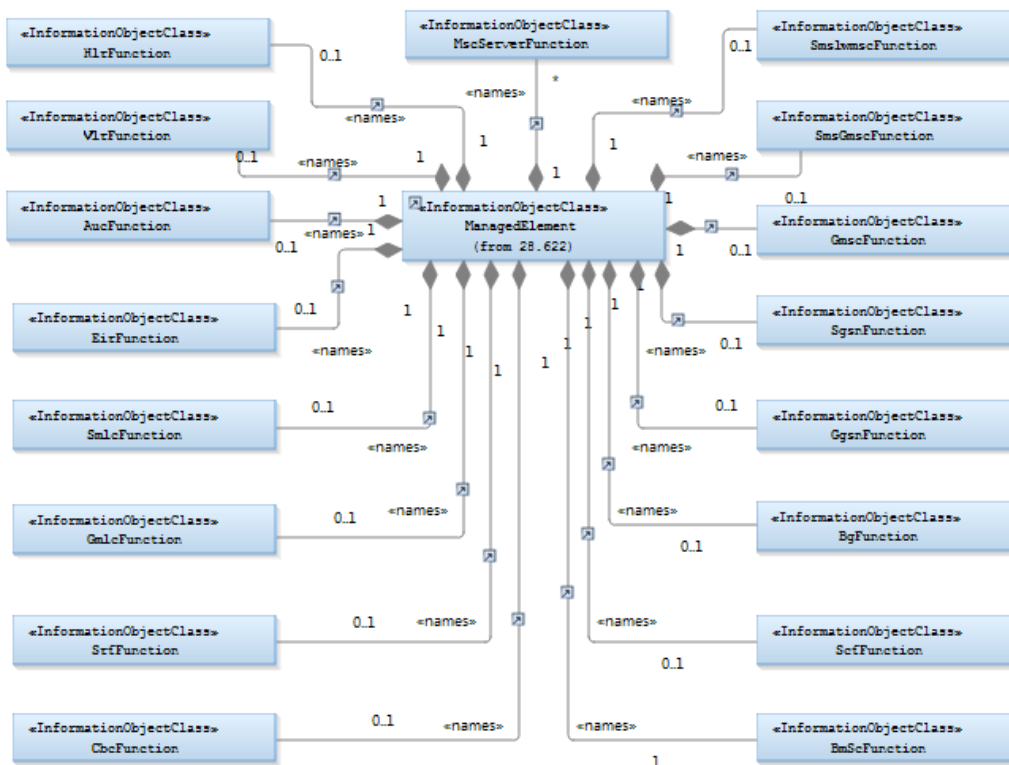
Figure 4.2.1.1: CN NRM Containment/Naming relationships 1
