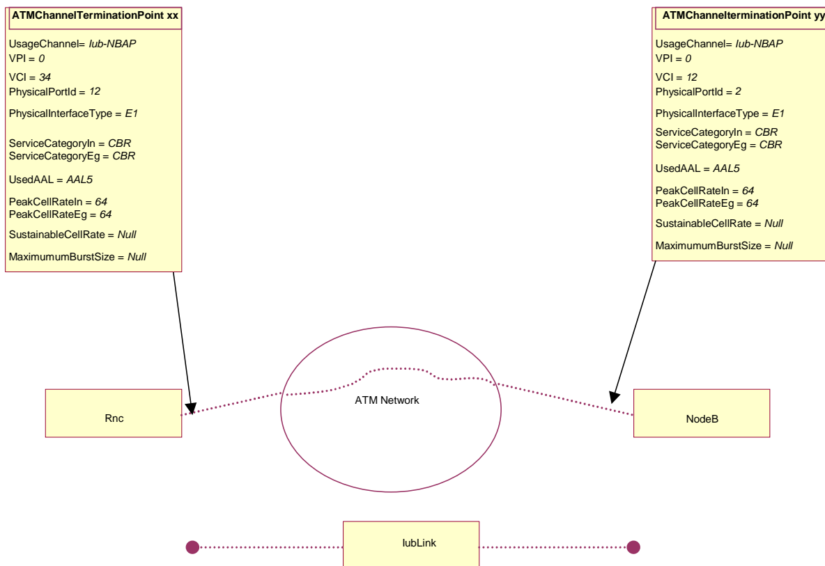
Figure A.1: Virtual connection of a logical lub interface channel over ATM network
