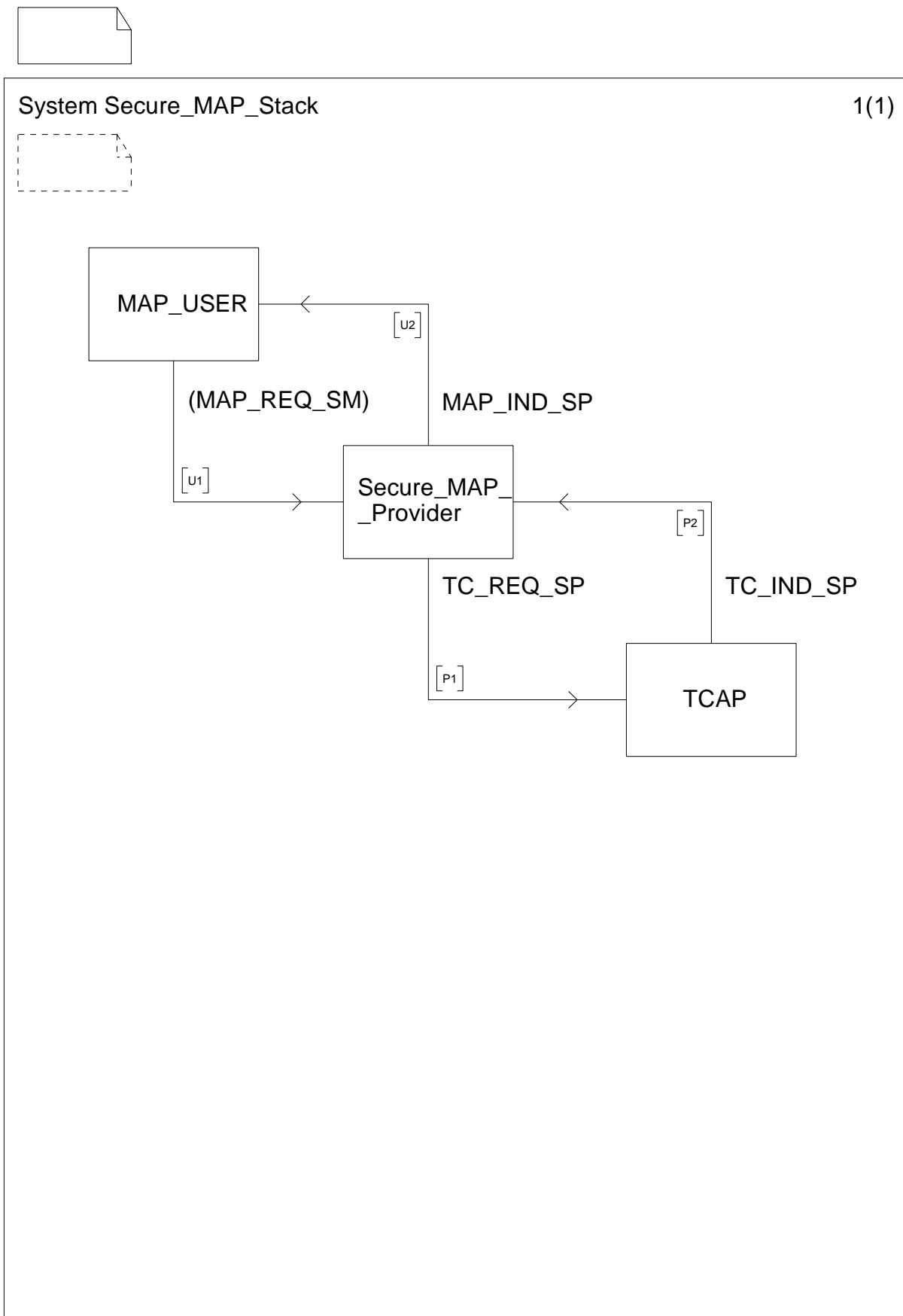
Figure 15.6/1: System Secure_MAP_Stack
