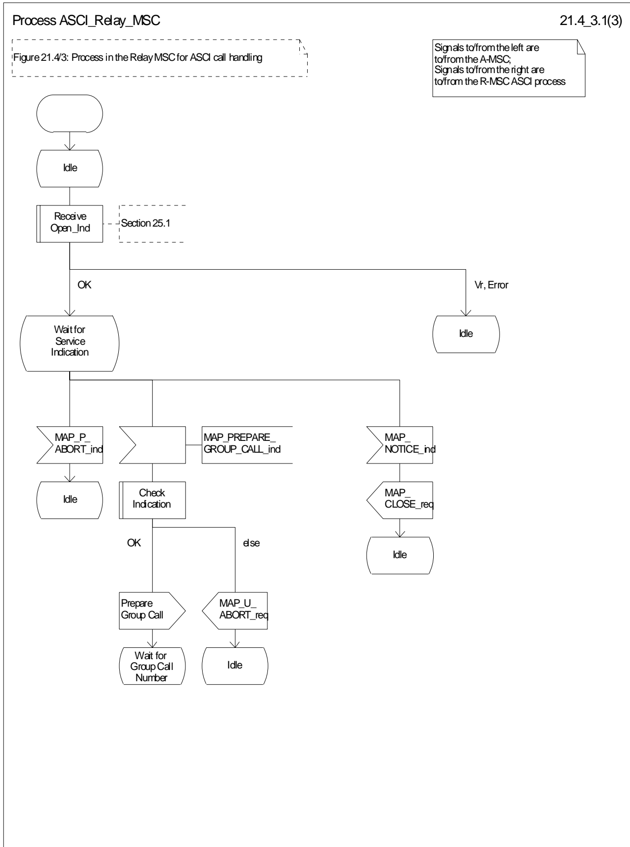
Figure 21.4/3 (sheet 1 of 3): Process ASCII_Relay_MSC
