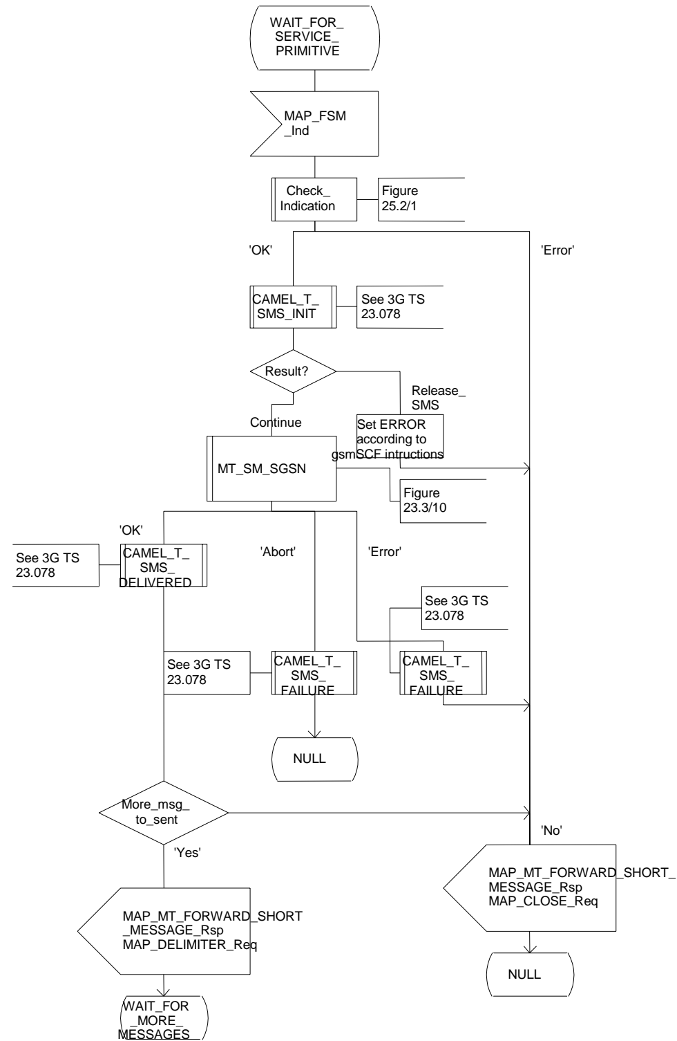
Figure 23.3/9: The mobile terminated short message service process in the SGSN
