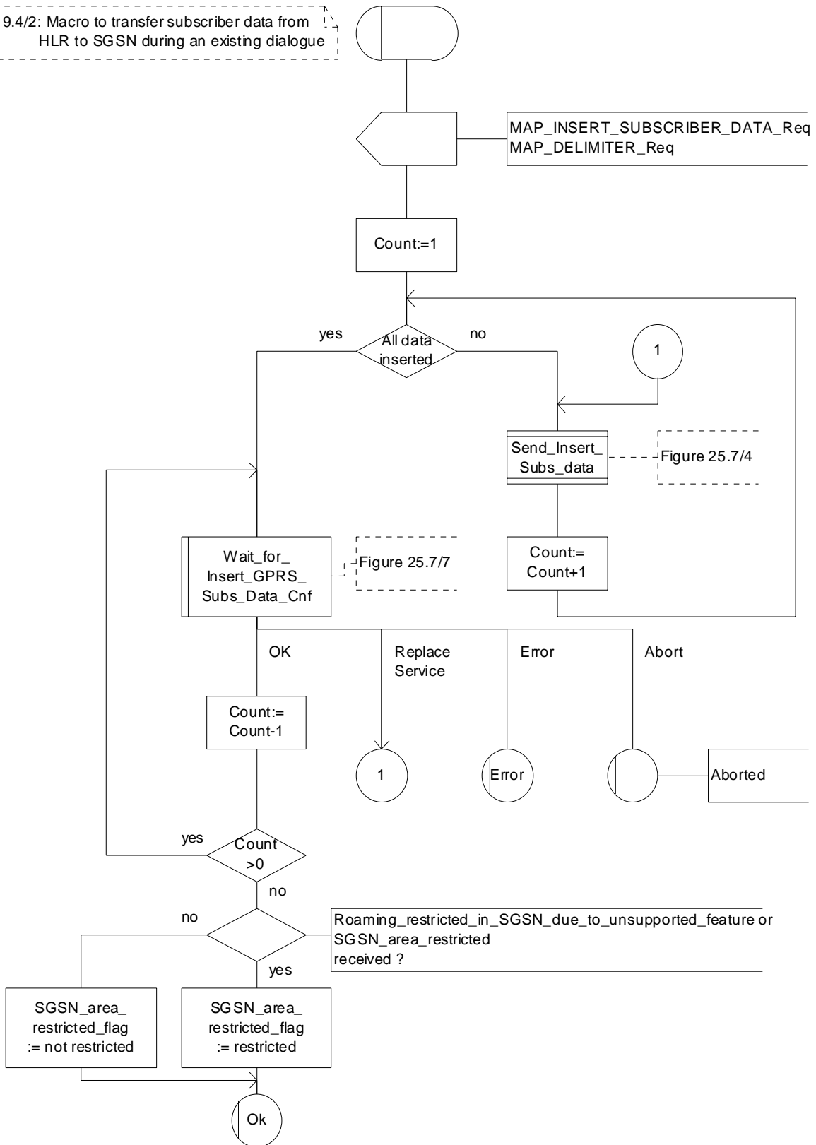
Figure 19.4/2: Macro Insert_Subs_Data_In_SGSN_Framed_HLR
