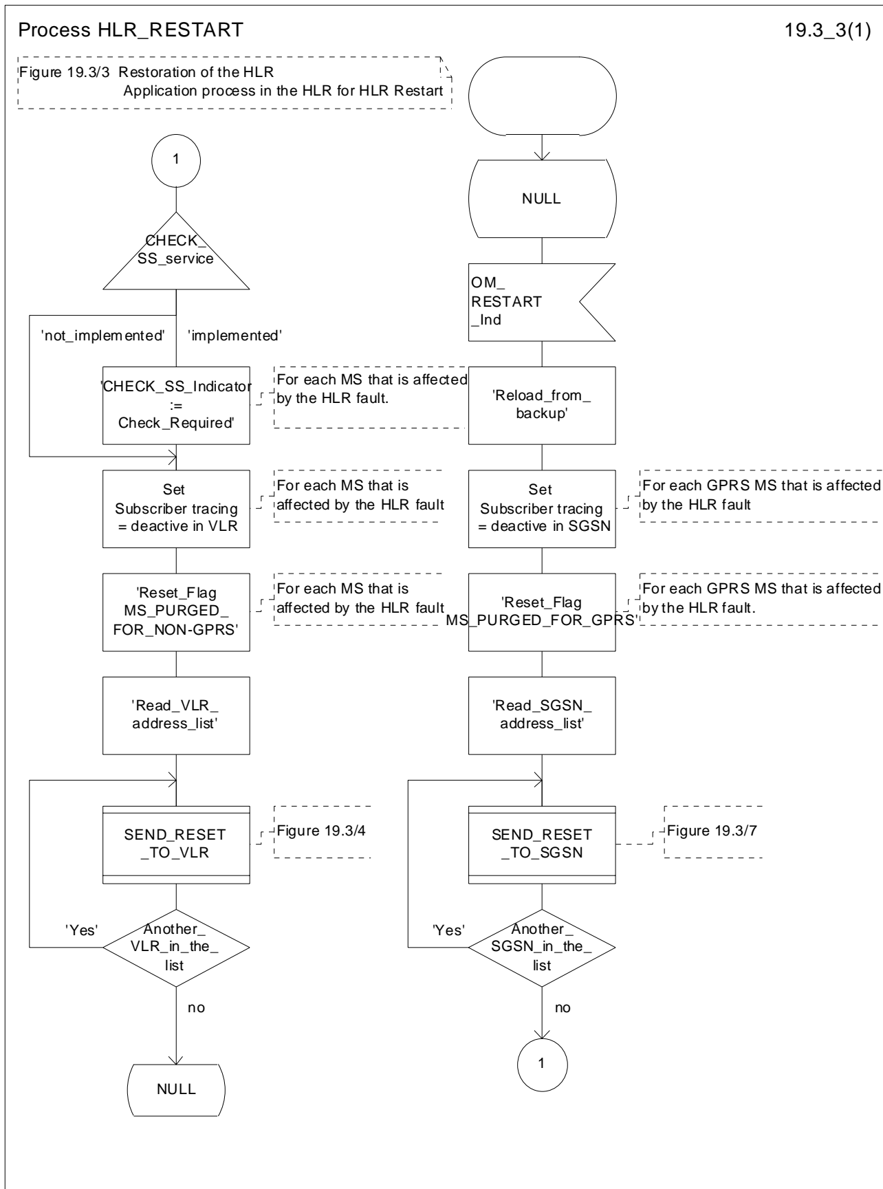
Figure 19.3/3: Process HLR_RESTART
