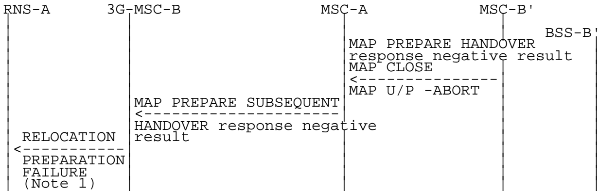
d) radio resources allocation failure:
