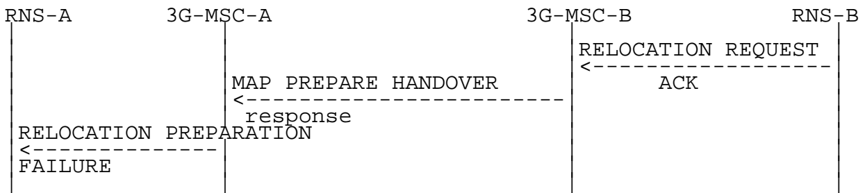
d) unsuccessful relocation execution (relocation cancelled):
