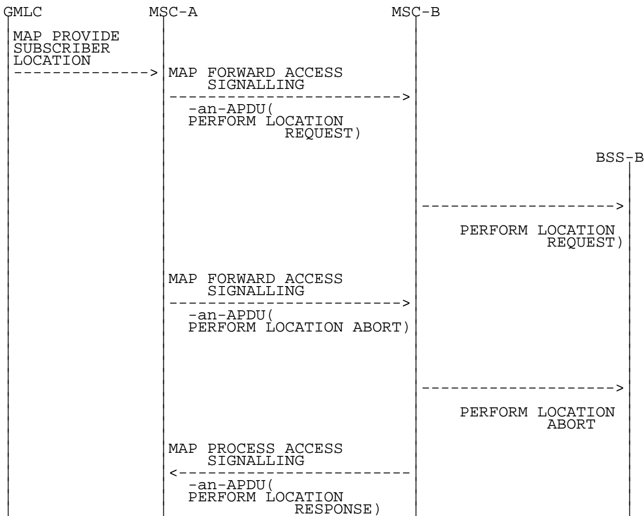
Figure 66a: Signalling for an aborted Location Acquisition procedure
