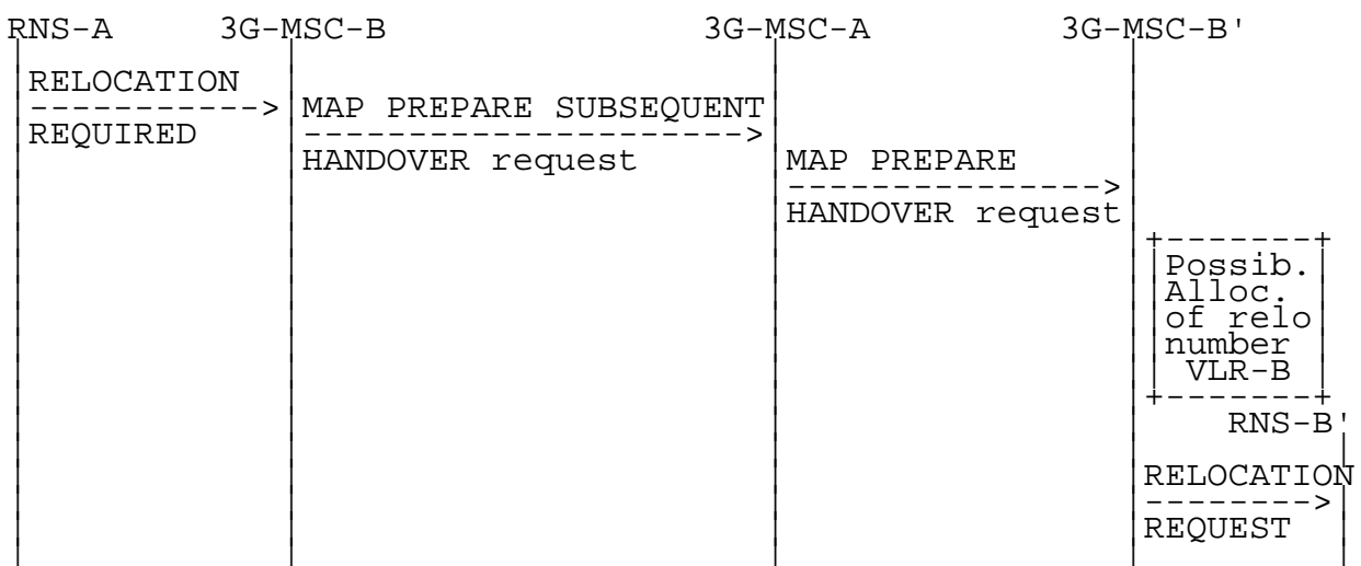
Figure 60: Signalling for Subsequent Inter-MSK Relocation to third MSC (3G_MSC-B') initiation
