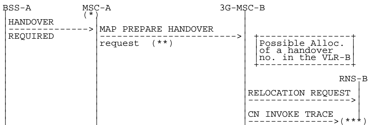
Figure 37b: Signalling for Basic Inter-MS-C Handover initiation (CN invoke trace message transferred)
