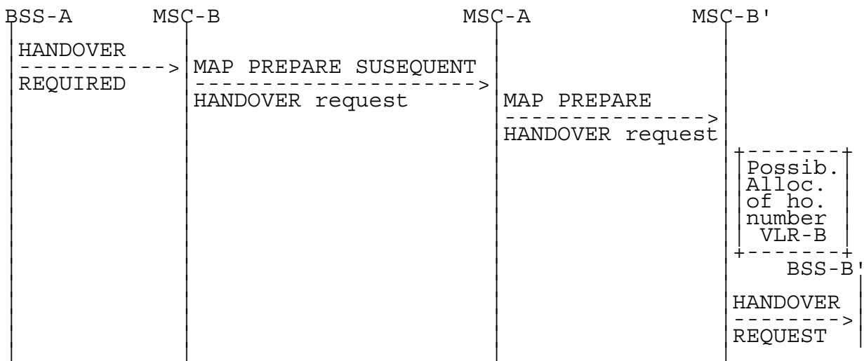
Figure 16: Signalling for Subsequent Inter-MS-C Handover to third MS-C (MS-C') initiation
