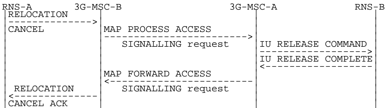
Figure 57: Signalling for Subsequent Inter-MSB Relocation back to 3G_MSC-A execution (Negative outcome)
