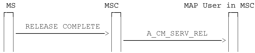
Figure 6.5: Signalling flow for SS connection release by the MS
