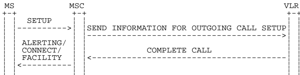
Figure 5.5: Signalling for notification of invocation of Call Forwarding supplementary service
